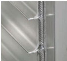
Interlocking aluminum extrusions with guides spaced on 1½" centers
