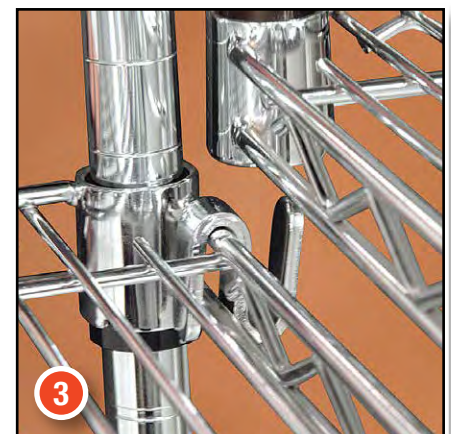
Two "S-Hooks" are used to connect add-on wire shelf to starter units.
