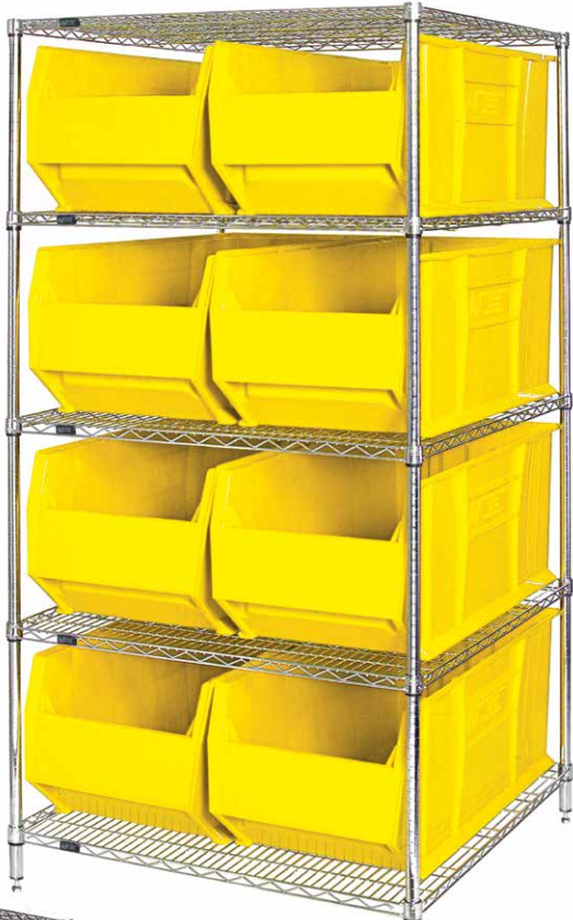
WR5-995 36"W x 48"L x 86"H 5 shelves and 8 QUS995 35-7/8"L x 19-7/8"W x 17-1/2"H bins
